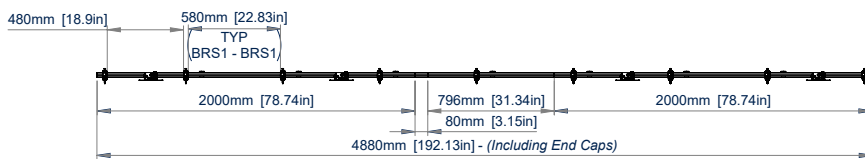
BOTTOM VIEW
