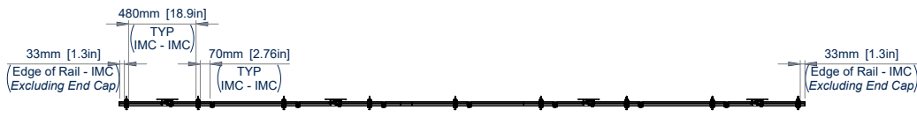
TOP VIEW
