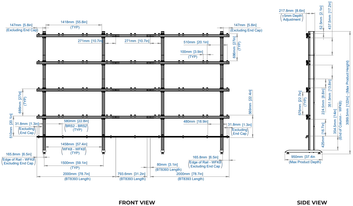
FRONT VIEW
