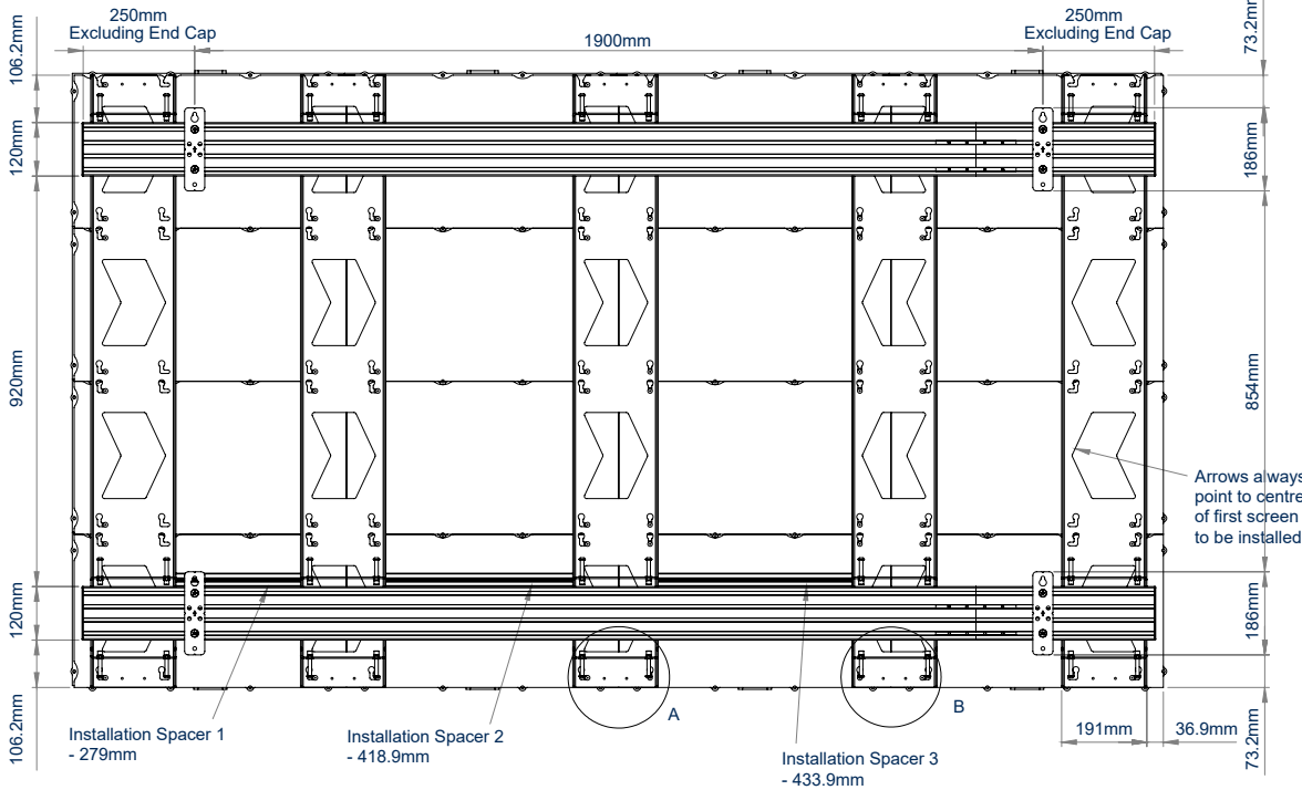
REAR VIEW
