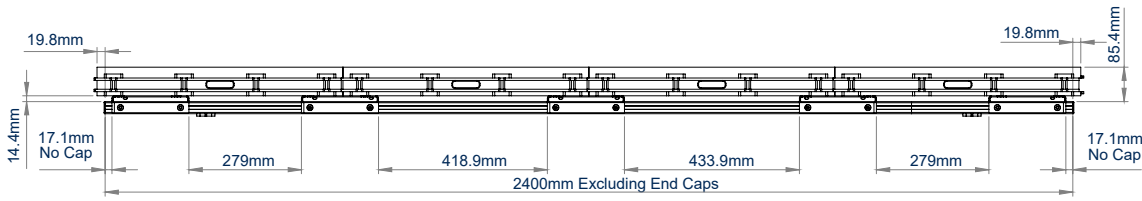
TOP VIEW
