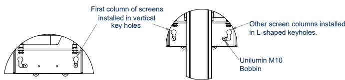
REAR VIEW
