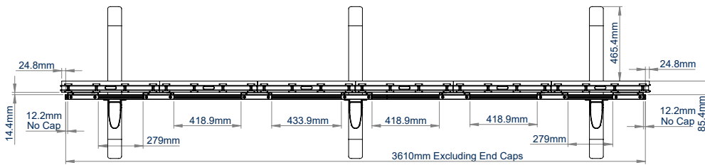
TOP VIEW
