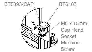
DETAIL D SCALE 1 : 5
