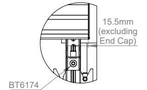
BT6174 DETAIL B SCALE 1 : 5
