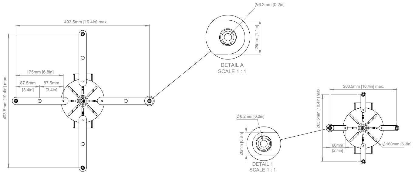
BOTTOM VIEW
