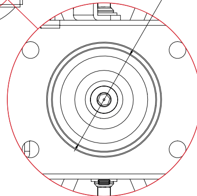
CEILING PLATE
