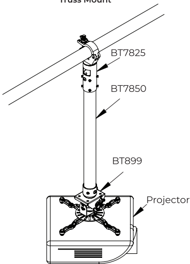
Truss Mount
