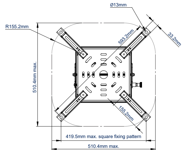
BOTTOM VIEW WITH SMALL EXTENSION LEGS
