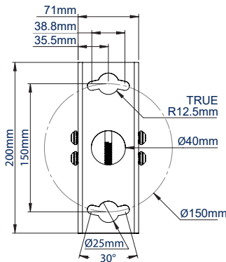
Ceiling / WALL PLATE
