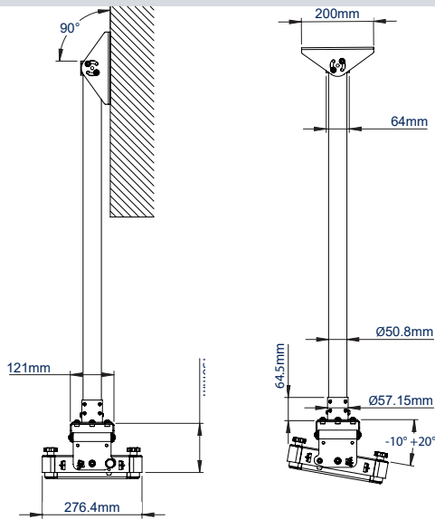
SIDE VIEW WALL MOUNTED
