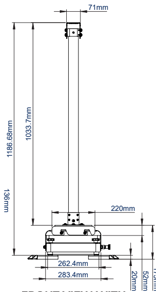
FRONT VIEW WITH EXTENSION LEGS
