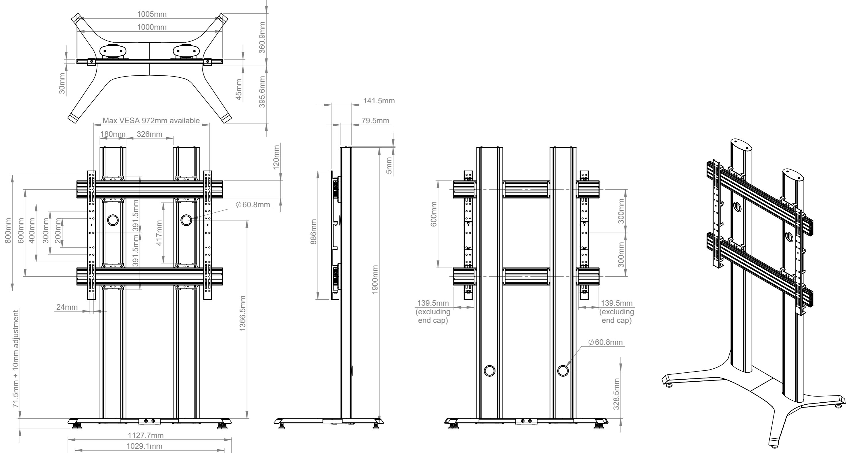
ISOMETRIC VIEW
