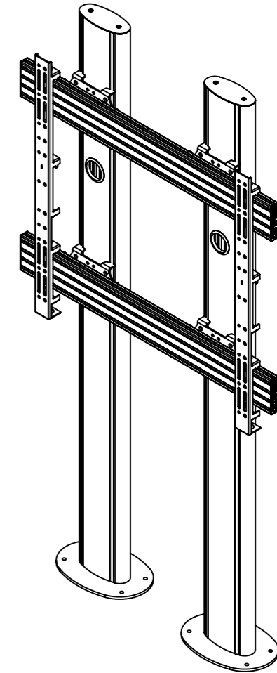
ISOMETRIC VIEW
