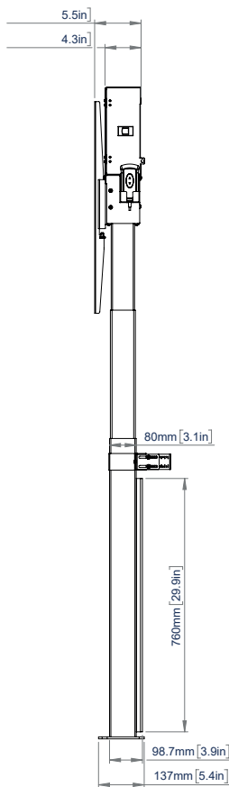
SIDE VIEW
