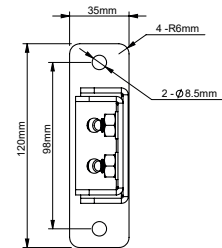
FRONT VIEW - WALL PLATE
