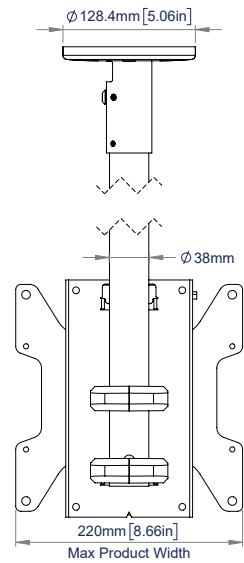
REAR VIEW
