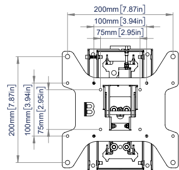
BT7611 MOUNTING PLATE
