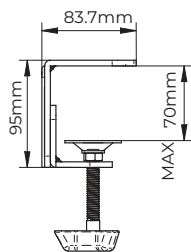
Desk Clamp
