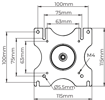
Interface Plate
