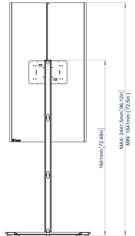
BACK VIEW
