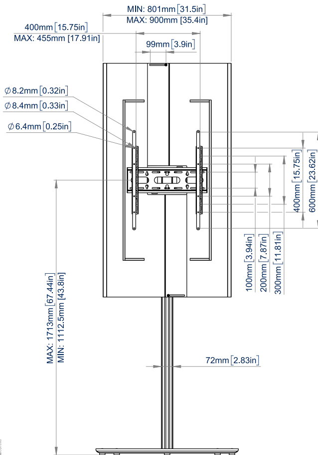
FRONT VIEW
