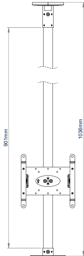
BT5964-FD200 FRONT VIEW
