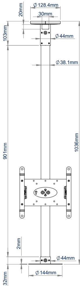
BT5964-FD100 FRONT VIEW
