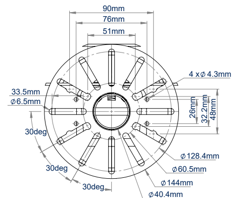
BOTTOM VIEW CCTV CAMERA MOUNT
