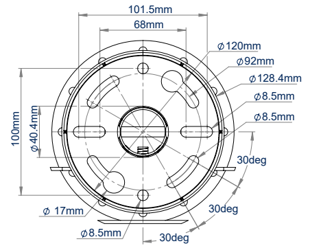
TOP VIEW CEILING PLATE
