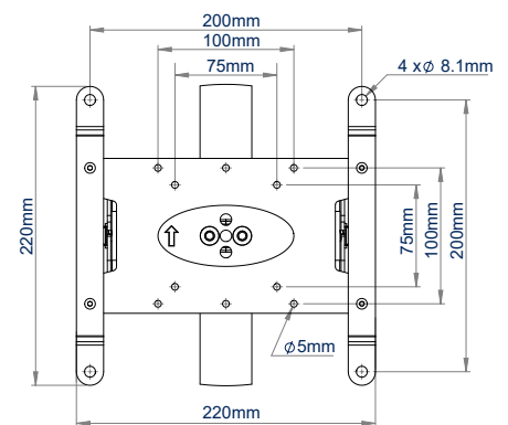
FRONT VIEW SCREEN MOUNT
