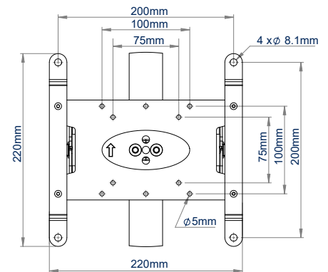
FRONT VIEW SCREEN MOUNT
