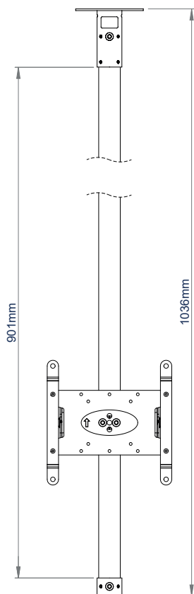
BT5964-FD200 VISTA FRONTAL
