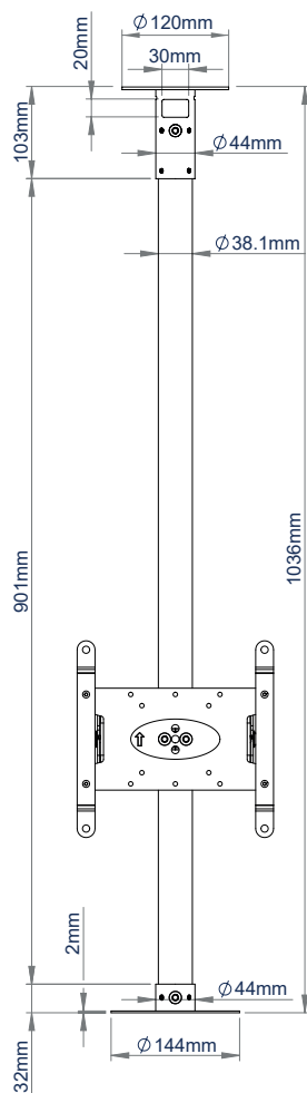
BT5964-FD100 VISTA FRONTAL
