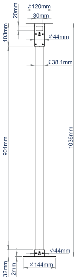
BT5960-FD100 VISTA FRONTAL
