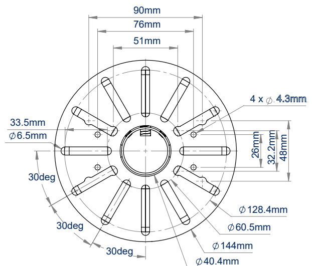
CEILING MOUNT TOP VIEW
