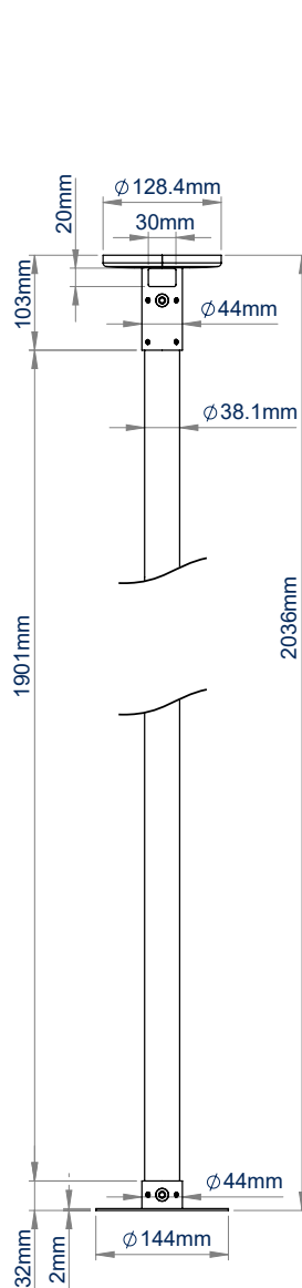
BT5960-FD200 FRONT VIEW
