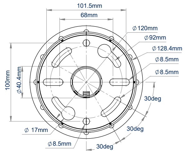
CEILING MOUNT TOP VIEW
