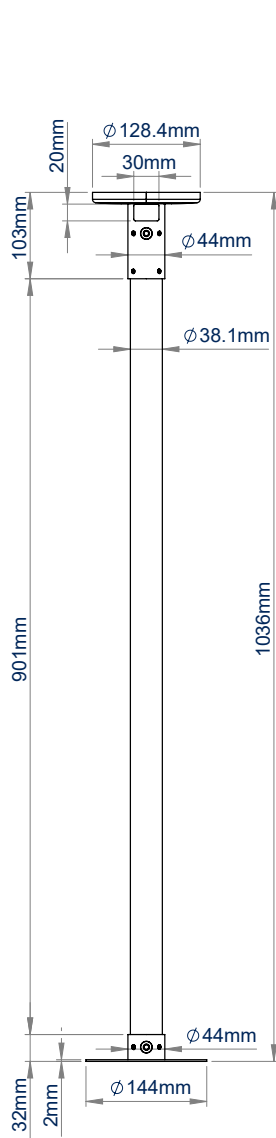
BT5960-FD100 FRONT VIEW
